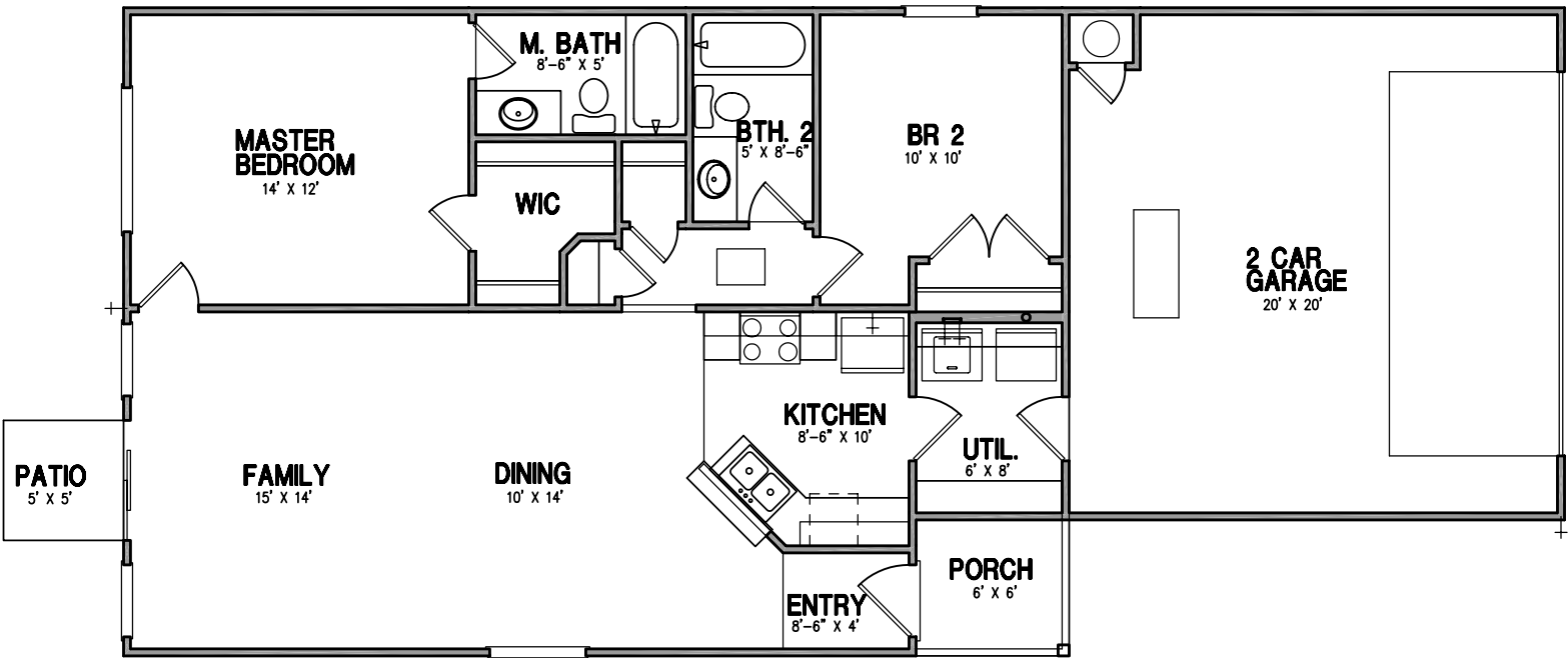
FLOOR PLAN
